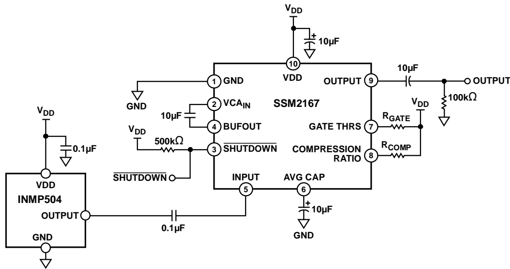
Figure 1. Analog MEMS Microphone Connection to Preamp
