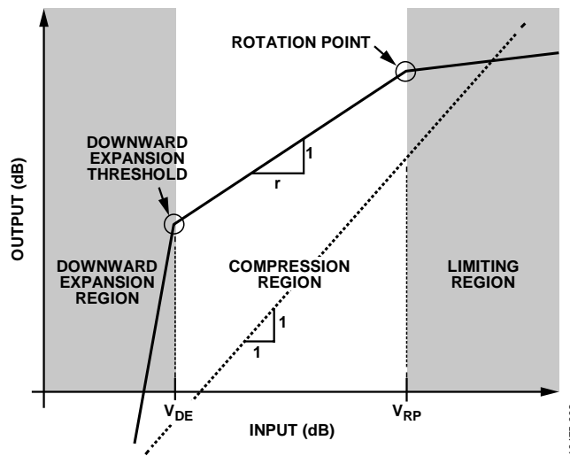
Figure 2. Gain Regions
