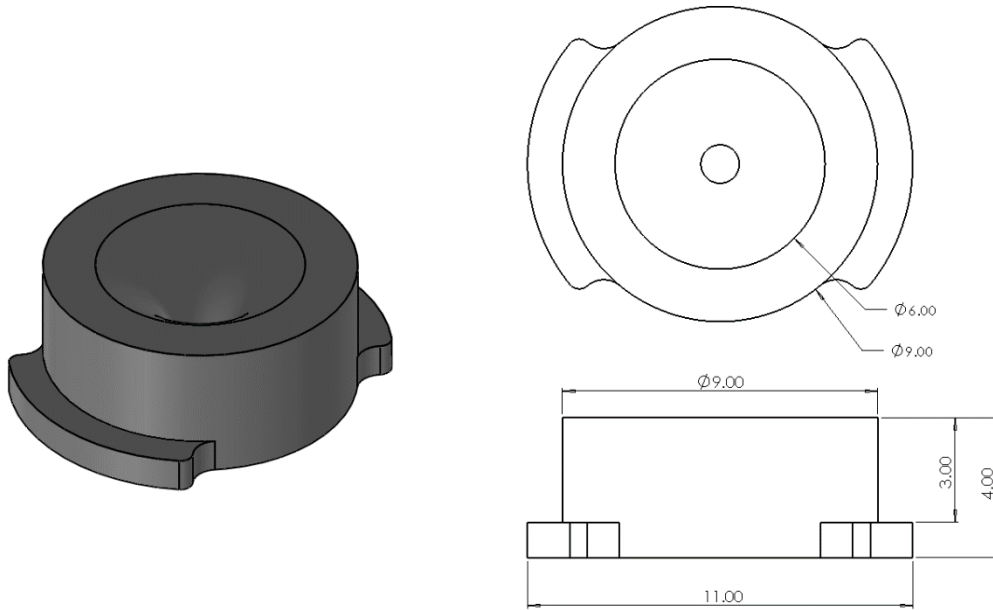
Figure 2: AH-20166-045045 Acoustic Horn Drawing
