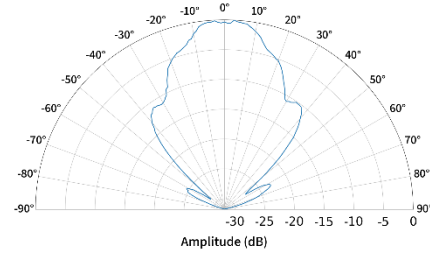
Figure 1: AH-20166-045045 Beam Patterns
