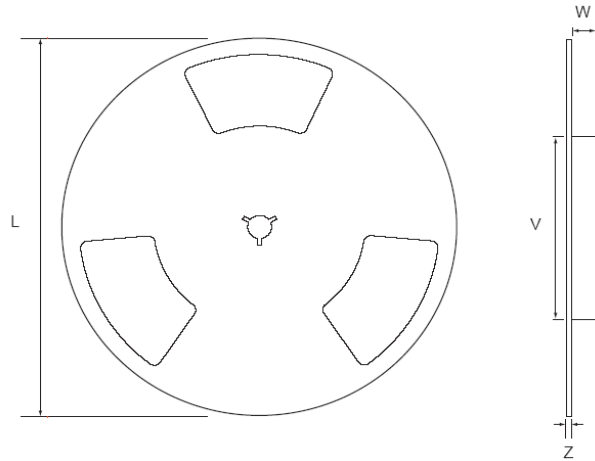
Figure 18. Reel Outline Drawing
