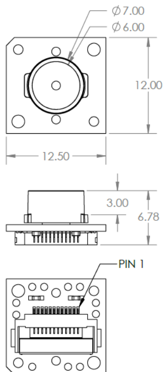
Figure 4. Dimensions of the EV_MOD_ICU-20201-01 Assembly
